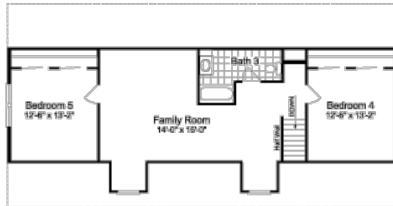
PROPOSED 2ND FLOOR Layout shown is for reference example only. All second floor layouts are by ethics and are required to meet the local codes.
