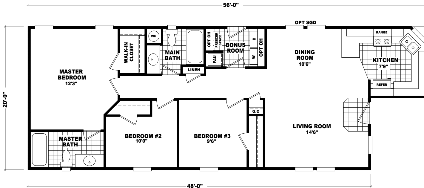
MODEL: GS-2560B APPROXIMATELY 1037 SQ. FT. 3 BEDROOM, 2 BATH
